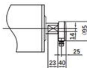
Elbow cable connector
