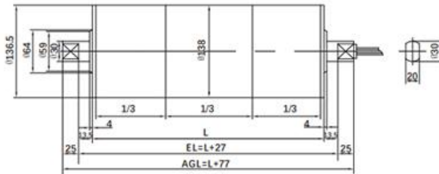
Straight cable connector
