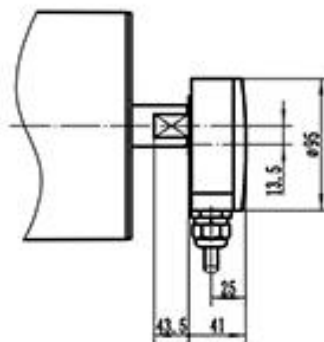
TM174H Idler roller
