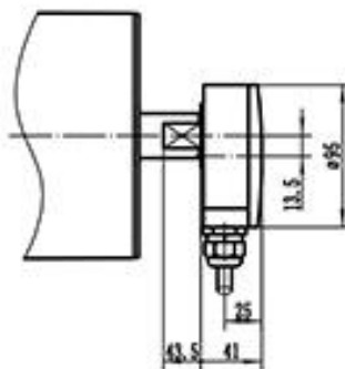
TM165H Idler roller
