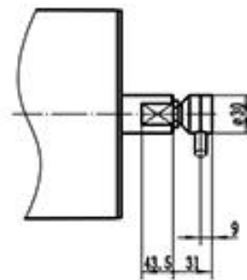
Elbow stainless steel cable connector
